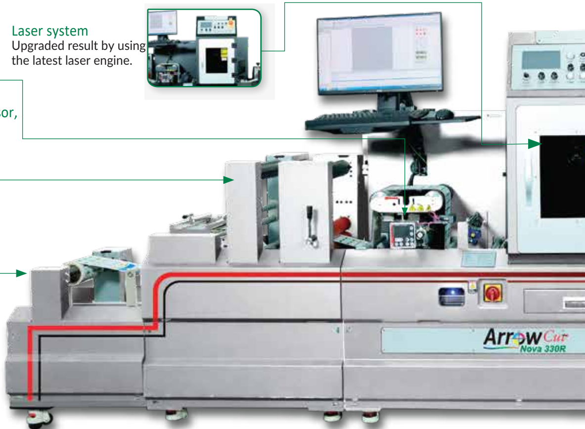
Unwinding system (350mm max web width / 400mm max roll diameter) Easy to install
